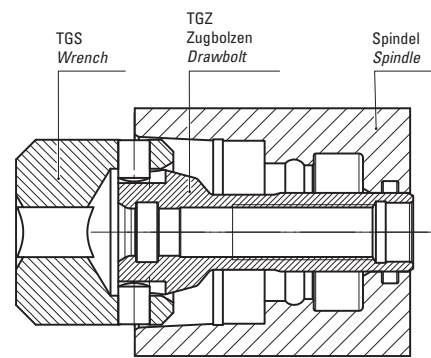
TGS Steckschlüssel
